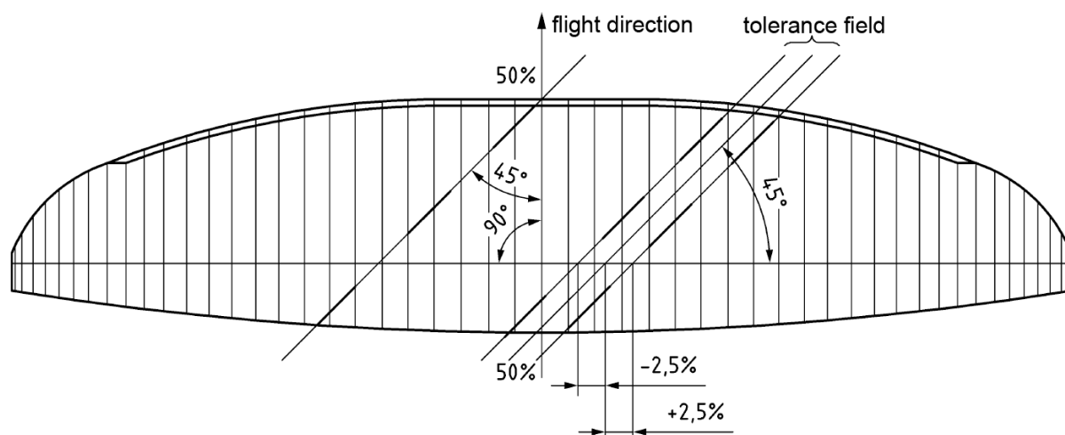
Figure 8: Canopy markingsControl lines
